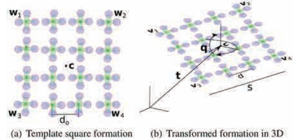
Fig. 5. (a) Example of a template square formation with sixteen MAVs. The four outer vertices define the convex hull. (b) The formation can be transformed with a translation \mathbf{t} , a 3D rotation \mathbf{q} and a size s isomorphic transformation.
