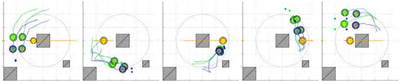
(a) Top view. From left to right, snapshots at 11 s, 20 s, 30 s, 37 s and 45 s, and paths of the robots in-between.
