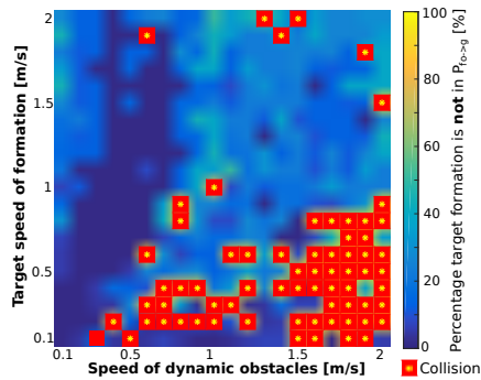
Fig. 4. Percentage of time in which the target formation, to make progress towards the goal, is within \mathcal{P}_{o \rightarrow g} or \mathcal{P}_g , but not in \mathcal{P}_{f_o \rightarrow g} . Here, lower values are better, since they correspond to the percentage of time for which the formation might be broken. Results for 3D navigation in the scenario of Fig. 3 with four quadrotors and varying speed of the dynamic obstacles and the formation. Fixed time horizon of \tau = 4 s is used in all experiments.
