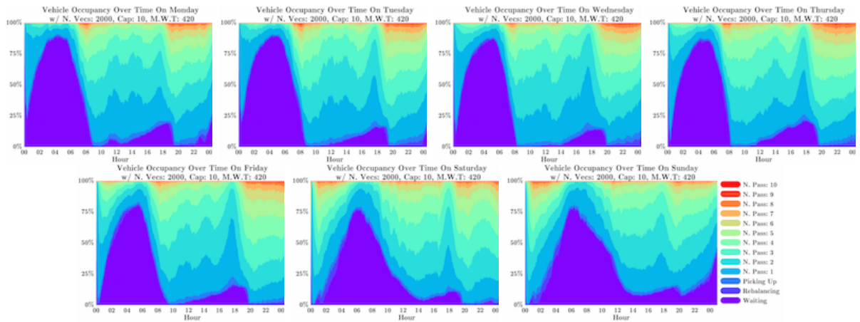
Fig. 30. Occupancy rates, 2000 vehicles, capacity 10, \Delta = 420 s
