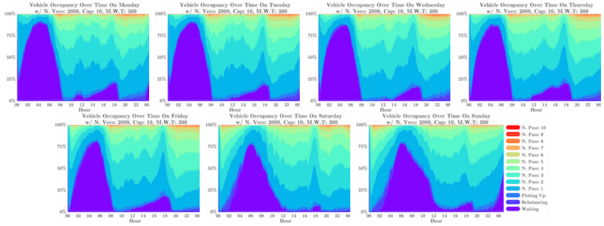
Fig. 29. Occupancy rates, 2000 vehicles, capacity 10, \Delta = 300 s
