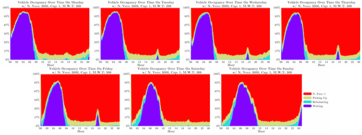
Fig. 32. Occupancy rates, 3000 vehicles, capacity 1, \Delta = 300 s
