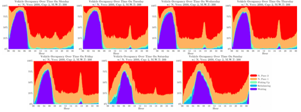
Fig. 23. Occupancy rates, 2000 vehicles, capacity 2, \Delta = 300 s
