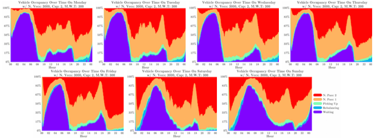
Fig. 35. Occupancy rates, 3000 vehicles, capacity 2, \Delta = 300 s
