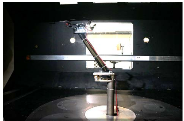
Figure 12: Quadrotor fixed in the wind tunnel
